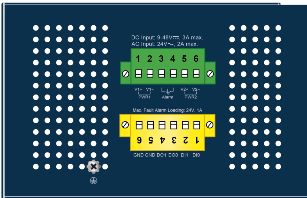
Figure 2-1-4d: Upper Panel of IGS-4215-24T4X
