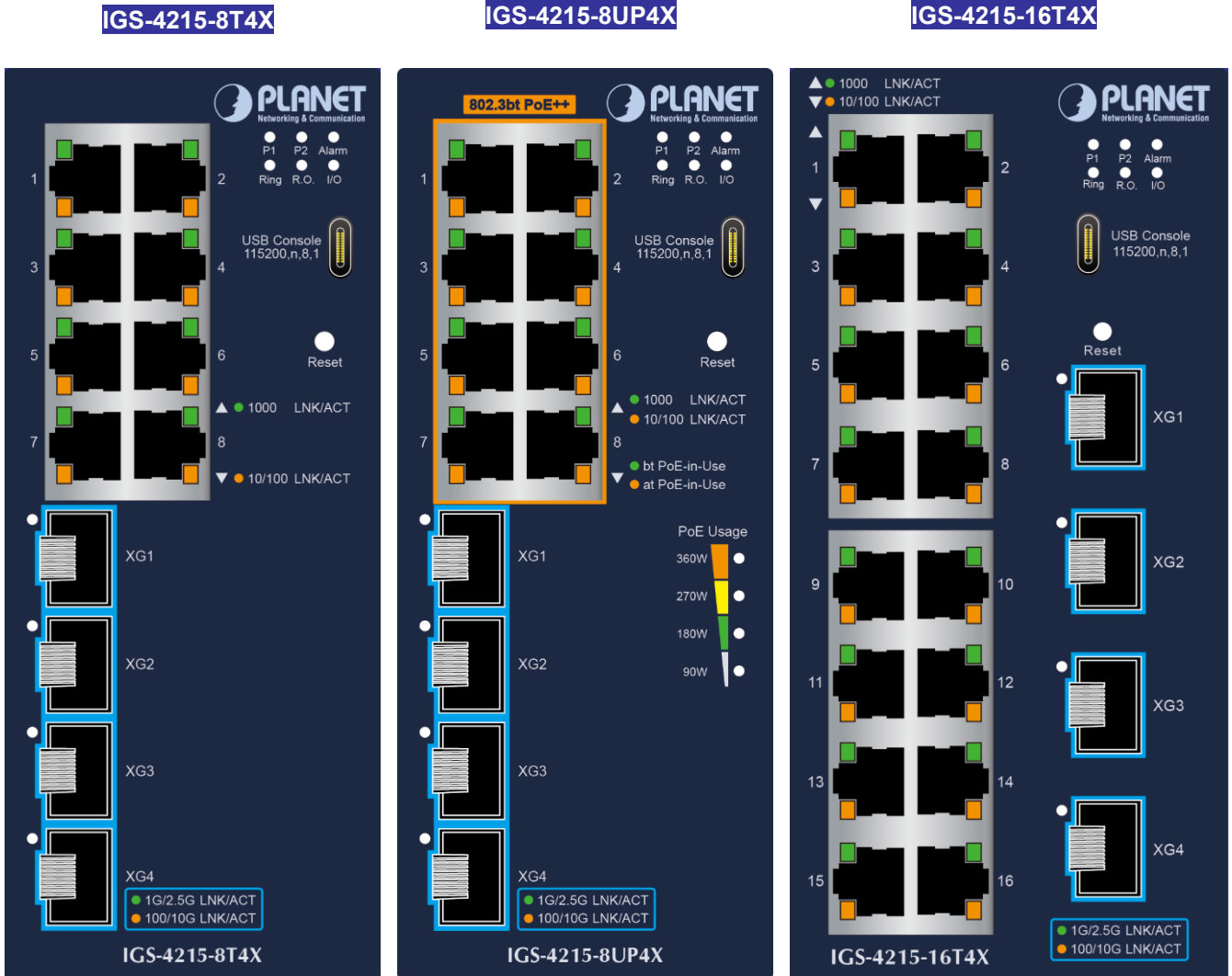
Figure 2-1-3a: IGS-4215-8T4X
