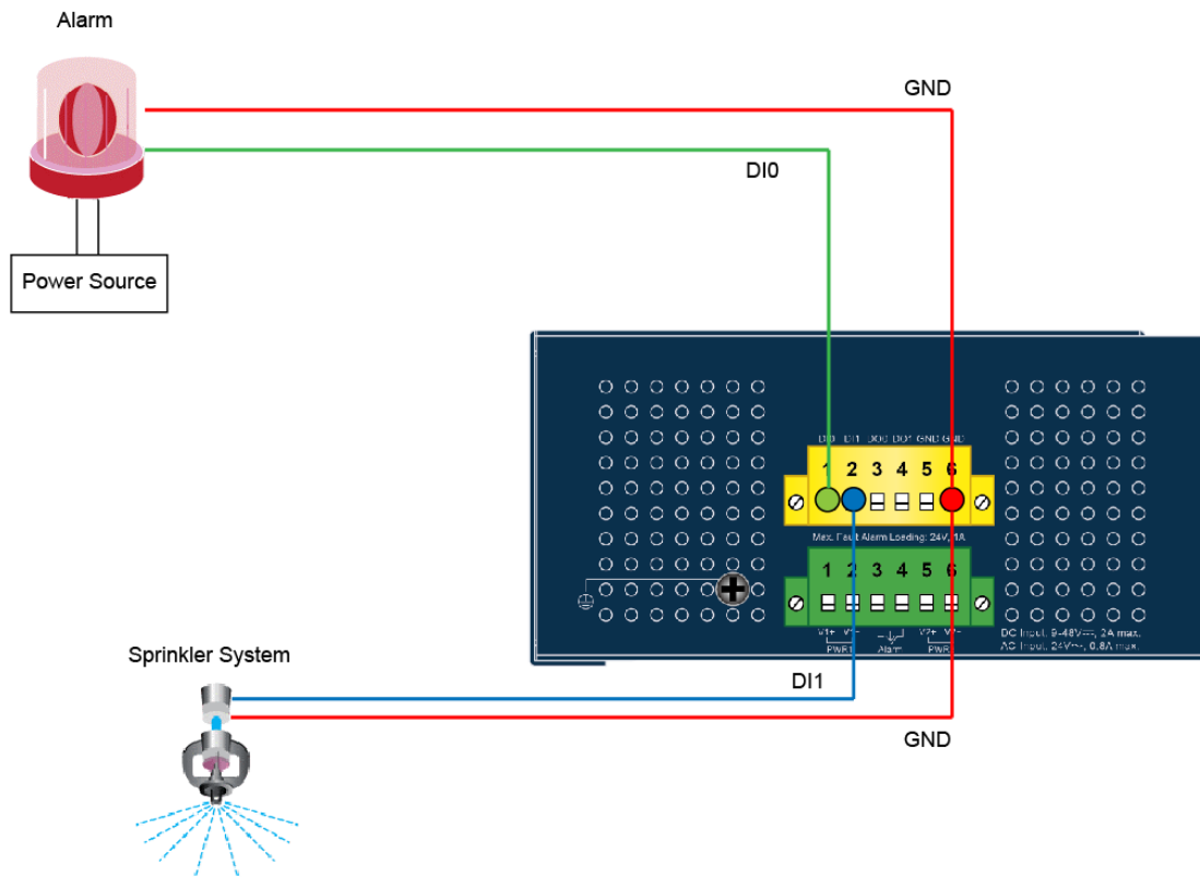
Figure 2-1-7d Wiring DO0 and DO1 to Open Detector
