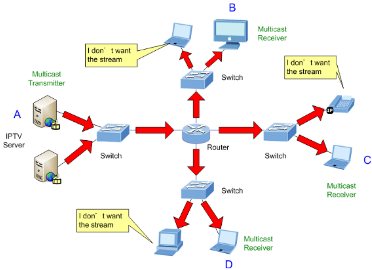
Figure 4-8-2: Multicast Flooding
