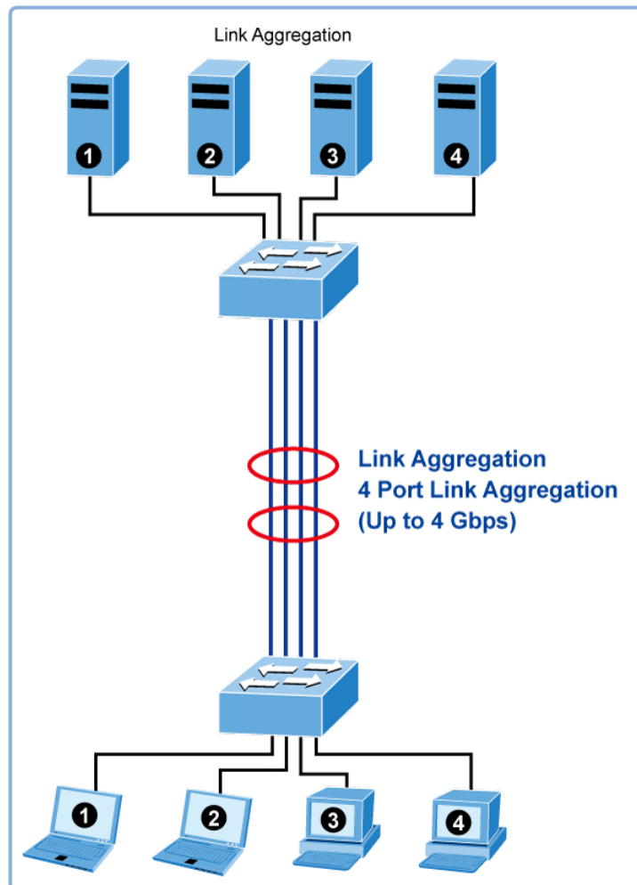
Figure 4-4-1: Link Aggregation
