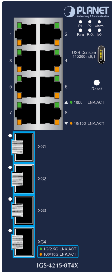
IGS-4215-8T4X
