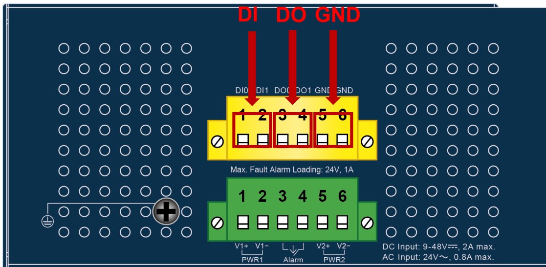
Figure 2-1-7a Wiring Digital Inputs/Outputs
