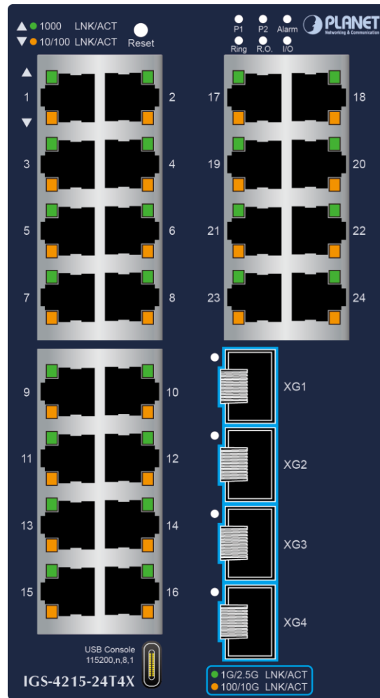
Figure 2-1-3d: IGS-4215-24T4X
