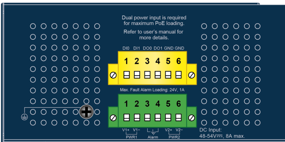
Figure 2-1-4b: Upper Panel of IGS-4215-8UP4X
