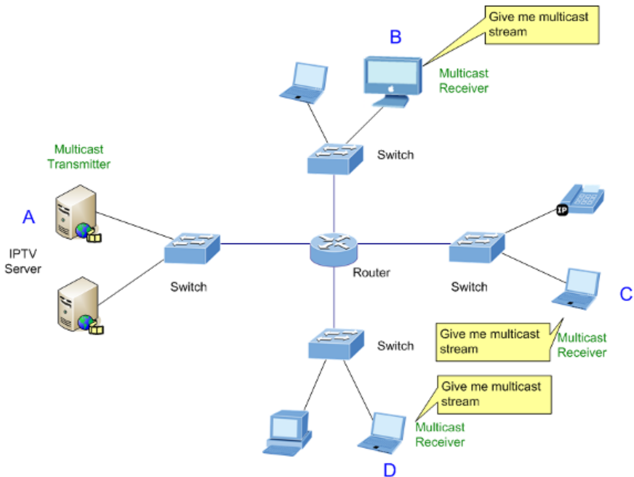
Figure 4-8-1: Multicast Service
