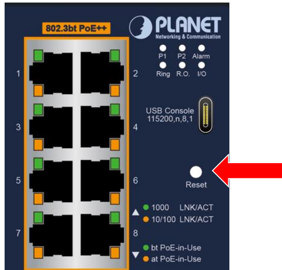
Reset button
