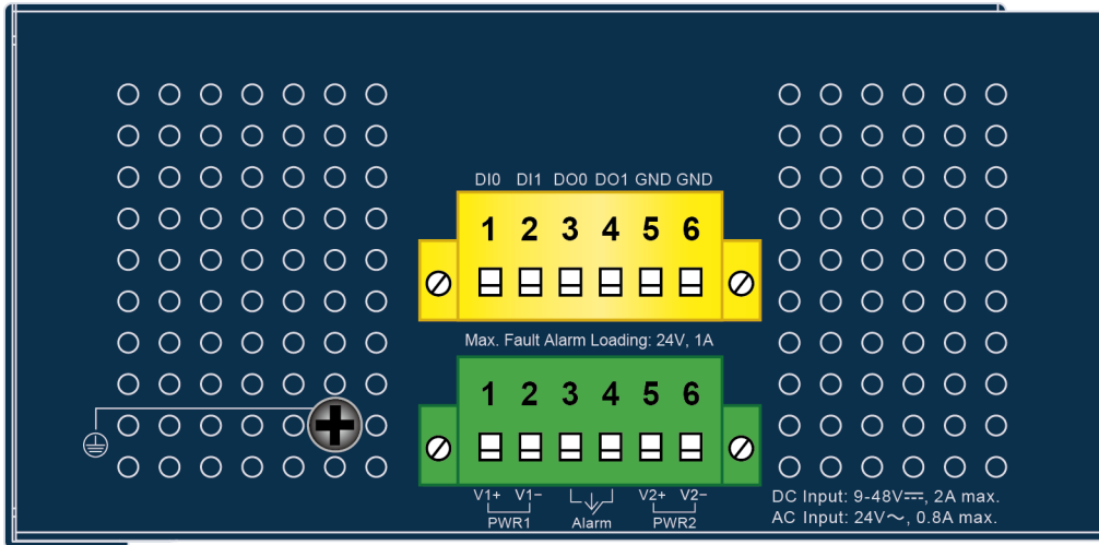
Figure 2-1-4a: Upper Panel of IGS-4215-8T4X
