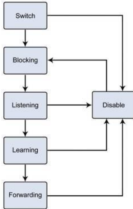
Figure 4-6-1: STP Port State Transitions
