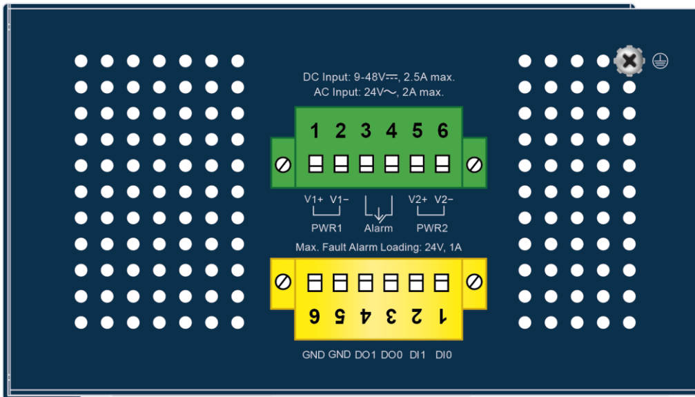
Figure 2-1-4c: Upper Panel of IGS-4215-16T4X
